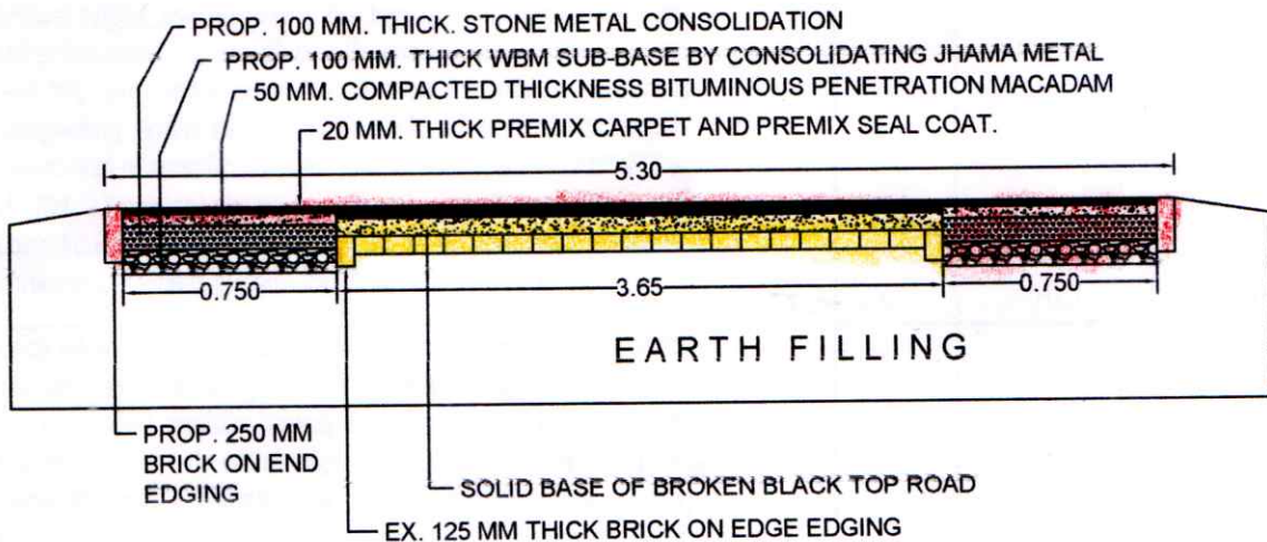
CROSS - SECTION OF ROAD Not to scale
